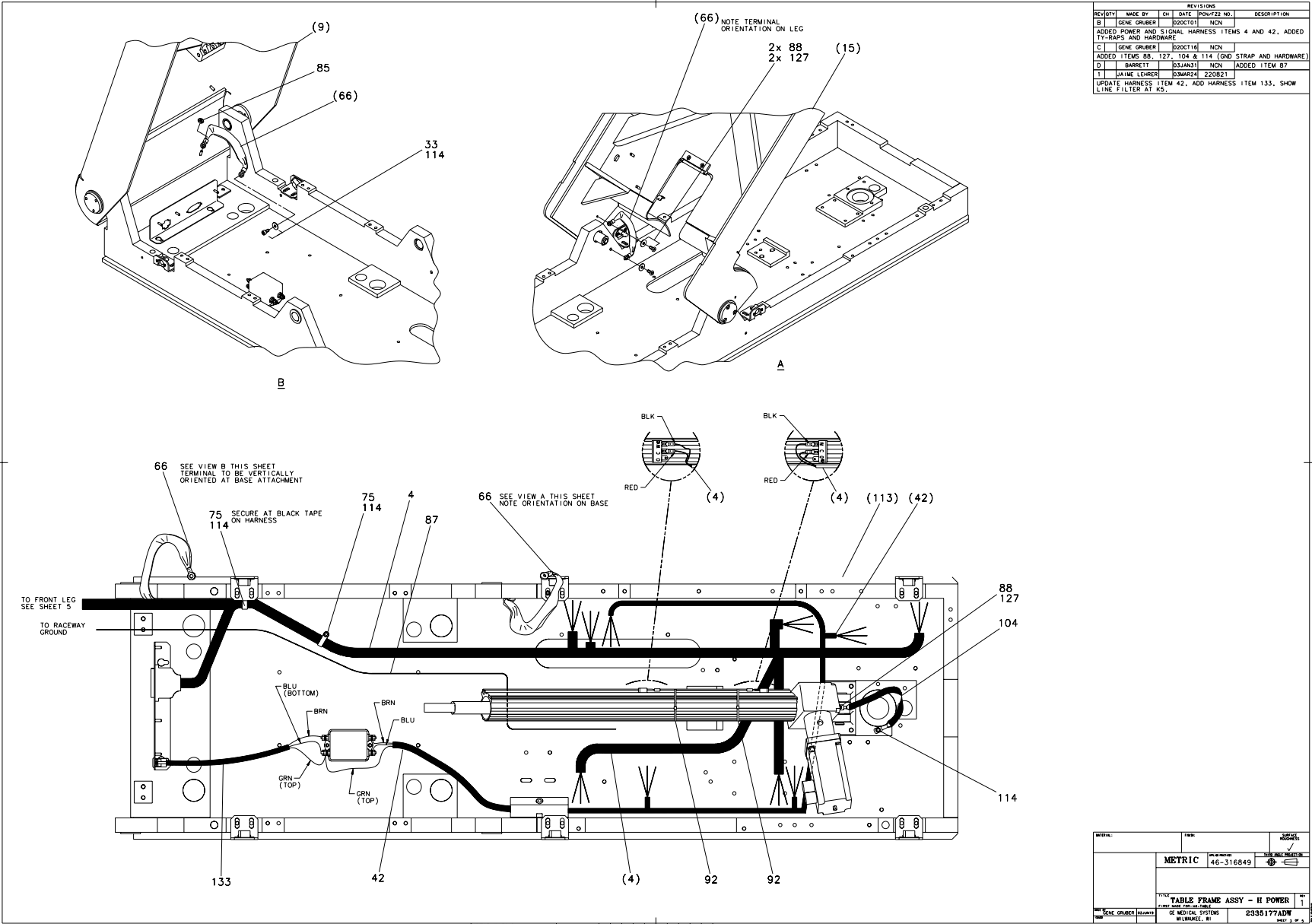
Figure 2-18 Table Frame Assembly (2335177, sheet 3, rev 1)
