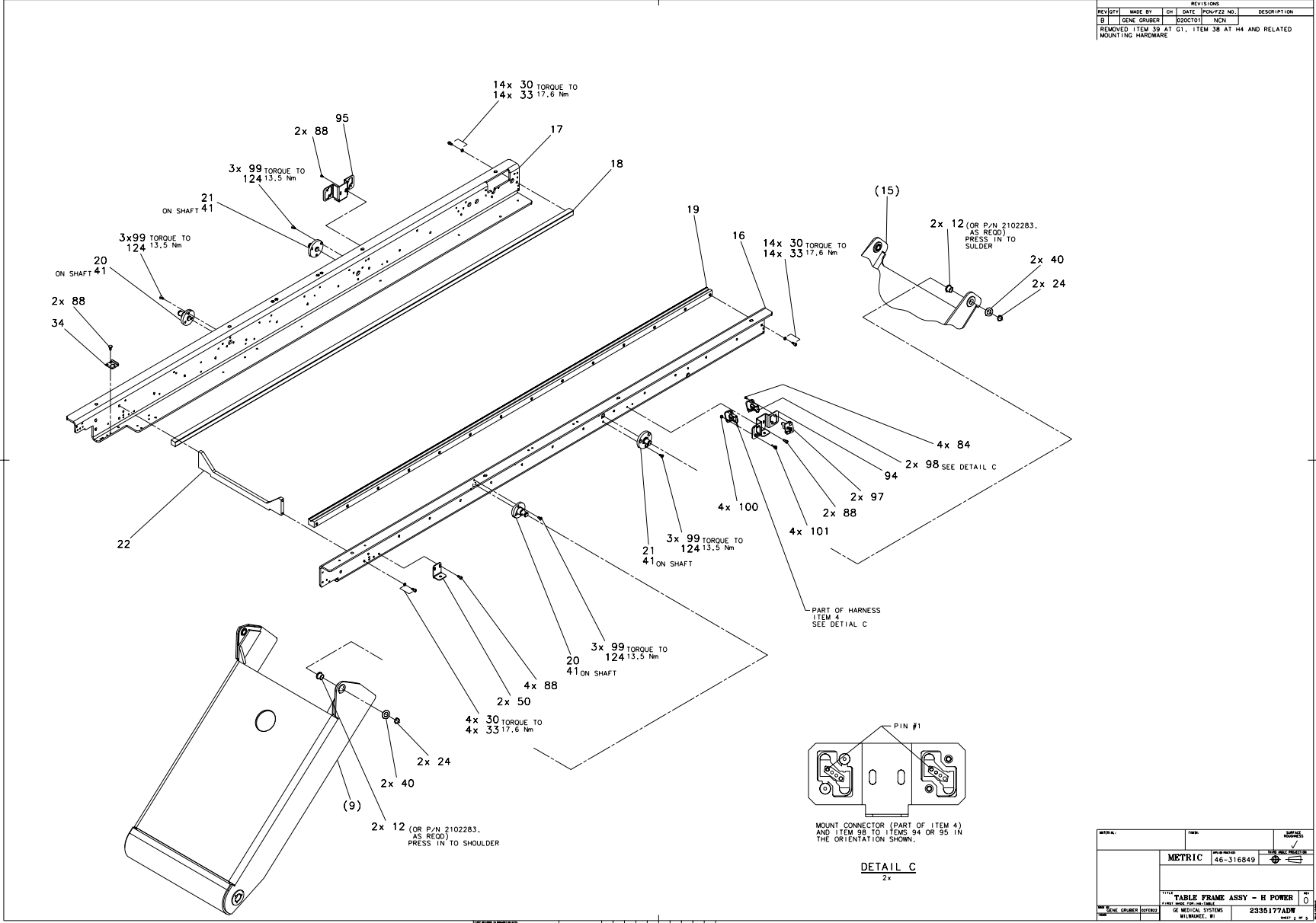
Figure 2-17 Table Frame Assembly (2335177, sheet 2, rev 0)
