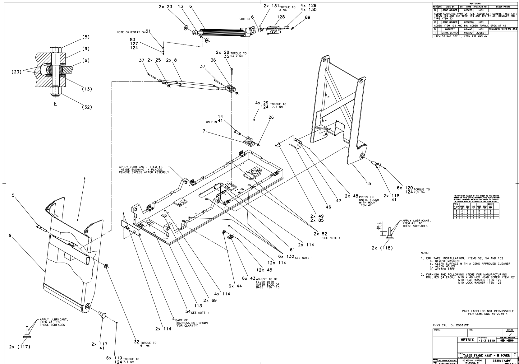
Figure 2-16 Table Frame Assembly (2335177, sheet 1, rev 1)
