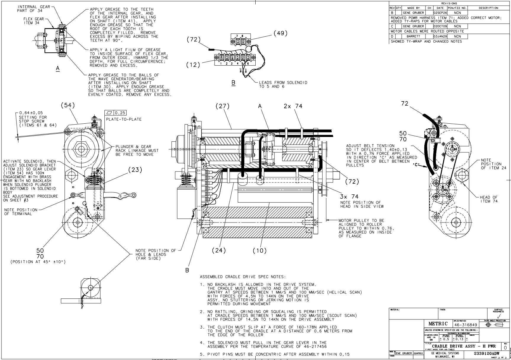
Figure 2-13 Cradle Drive Assembly (2339120, sheet 2, rev 0)
