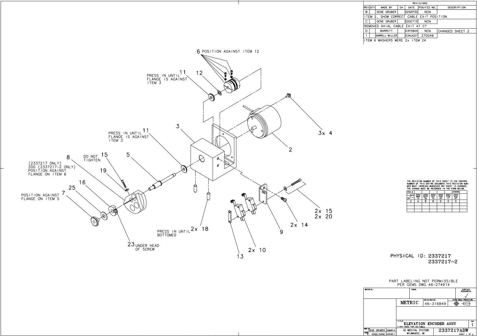
Figure 2-15 Encoder Assembly, Elevation - H Power (2337217, sheet 1, rev 1)
