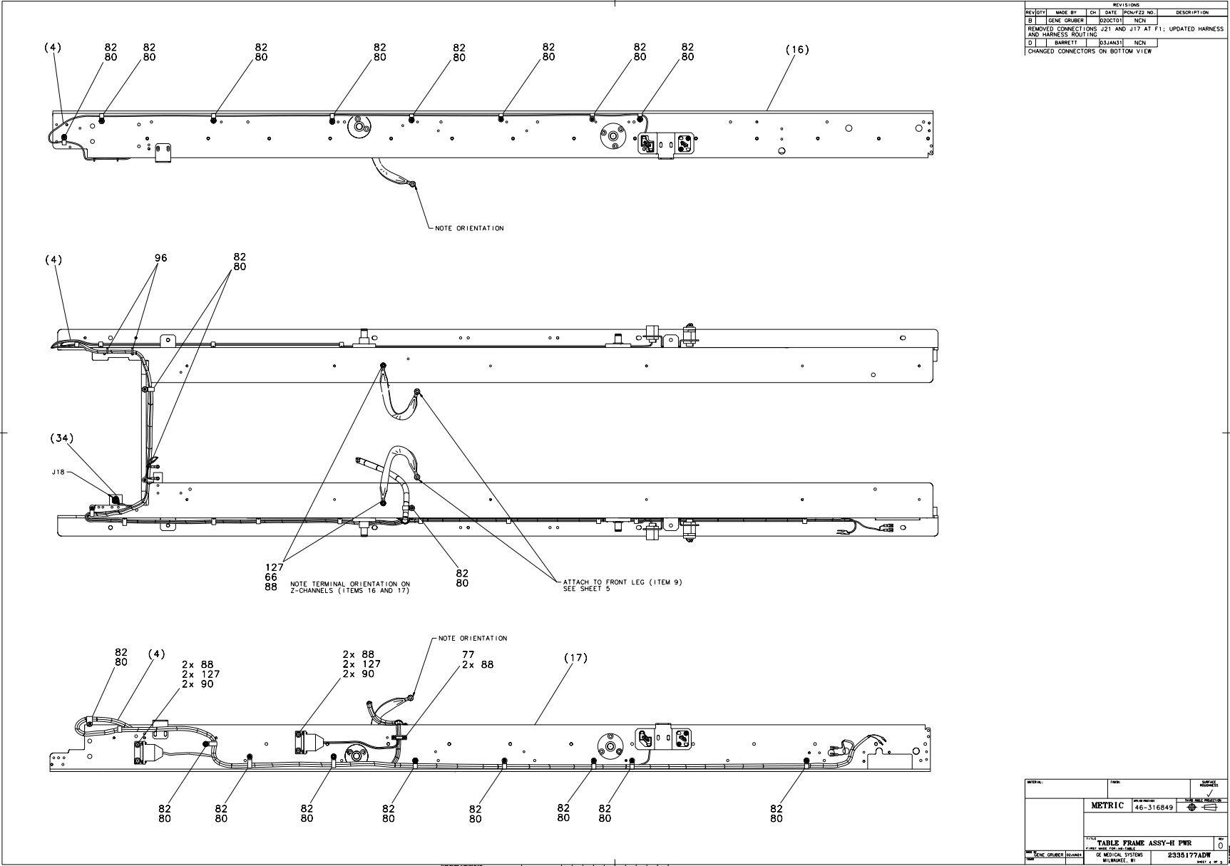
Figure 2-19 Table Frame Assembly (2335177, sheet 4, rev 0)
